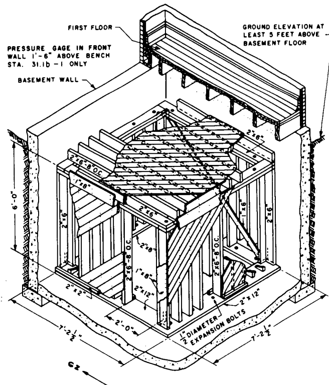
Fig. 6—Sketch of basement corner-room shelter.
